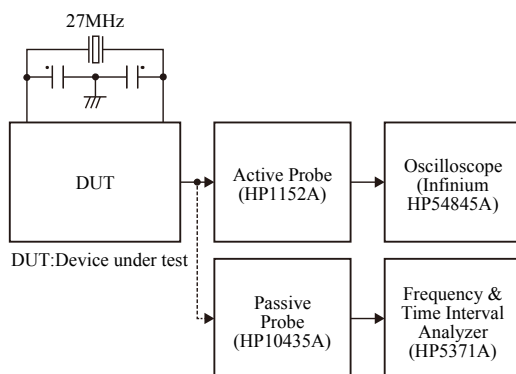
Figure 1. Measurement circuit 1
