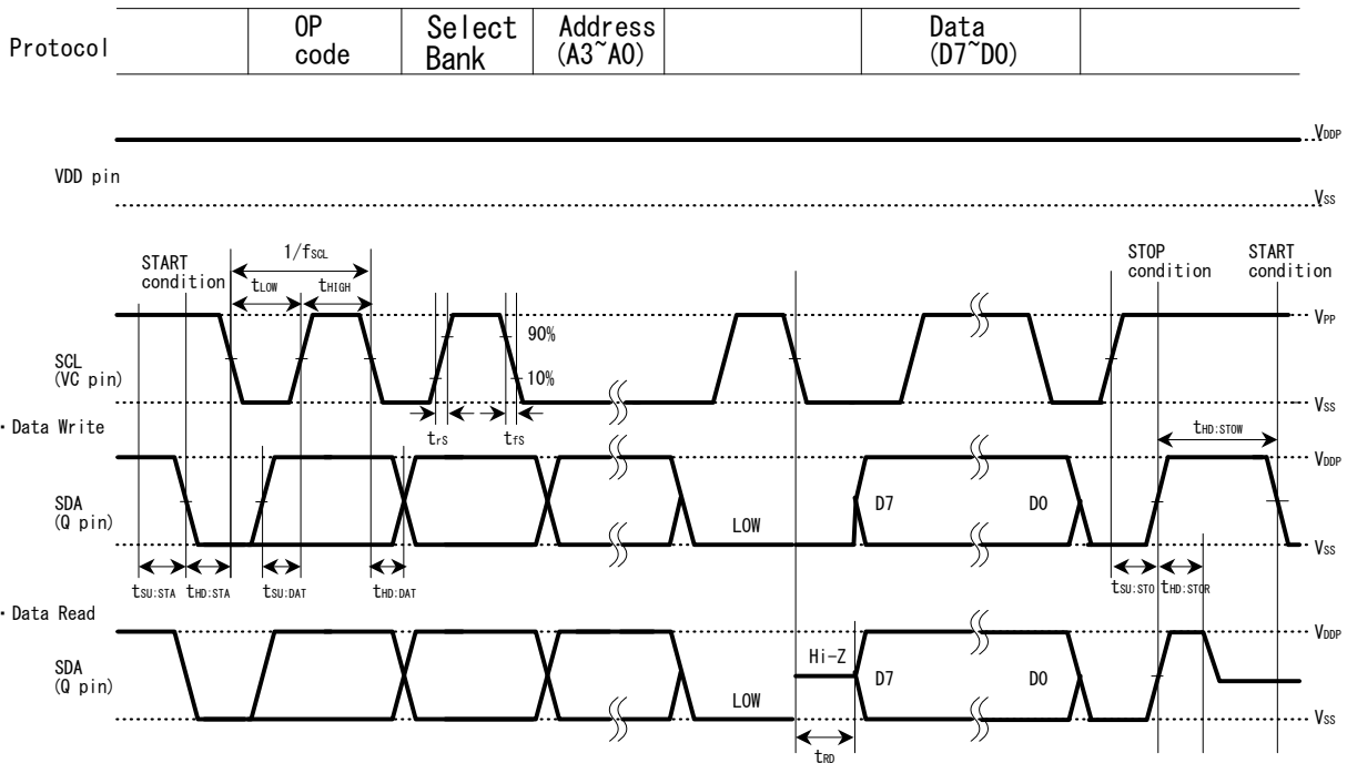
Serial interface timing diagrams
