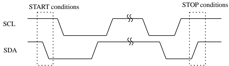
Programming start/stop condition waveform
