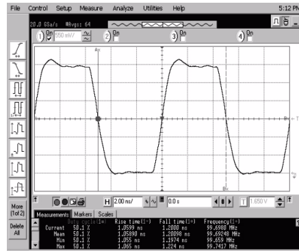
5027×D, V_{DD} = 3.3V , f_{OUT} = 100MHz , C_{LOUT} = 15pF , T_a = 25^\circ C
