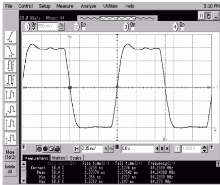
5027×D, V_{DD} = 3.3V , f_{OUT} = 85MHz , C_{LOUT} = 15pF , T_a = 25^\circ C
