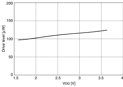
5027×D, f_{OUT} = 85\text{MHz} , T_a = 25^\circ\text{C}
